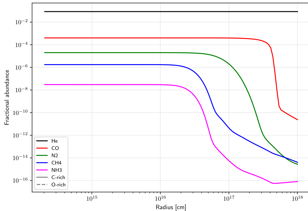
Fractional abundances - complete_model_Mdot1e-5_15kms_v2
