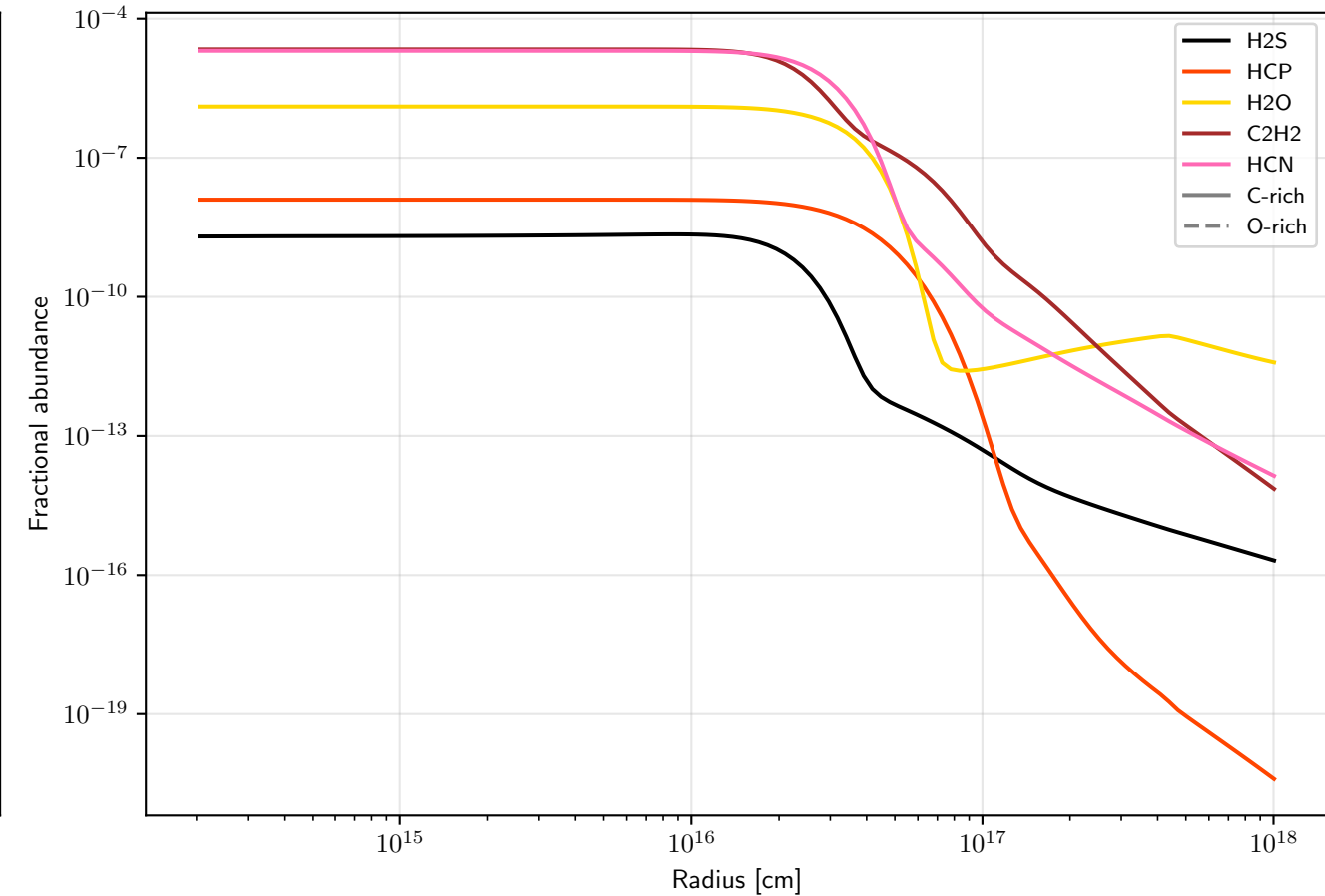
Fractional abundances - complete_model_Mdot1e-5_15kms_v2
